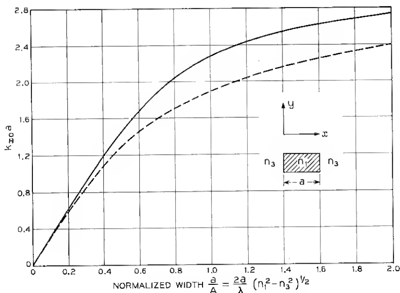
Fig. 3—Guide's electrical width. Solid line is for E_{11}^x mode with n_1/n_3 = 1.5 ; dashed line is for E_{11}^x mode with n_1/n_3 arbitrary, and for E_{11}^x mode with n_1 \cong n_3 .
