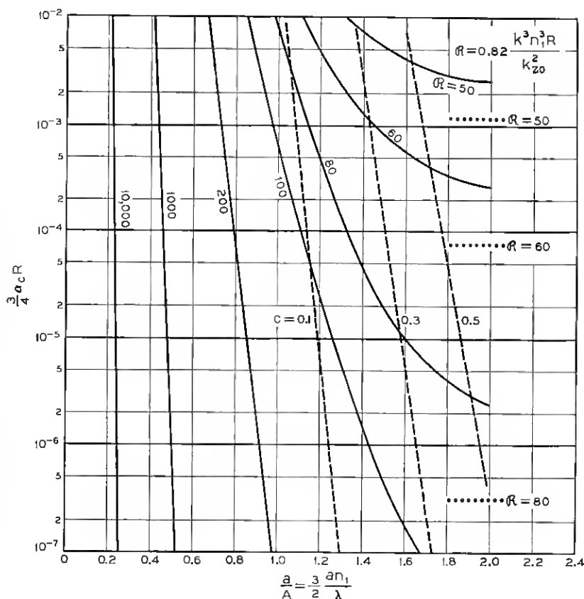
Fig. 5—Attenuation per radian for E_{11}^r mode if n_1/n_2 = 1.5 .
