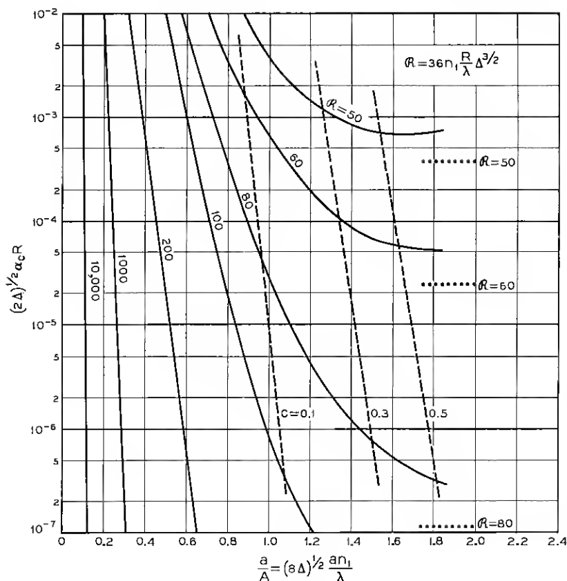
Fig. 4—Attenuation per radian for E_{1r}^s and E_{1r}^p modes if n_1/n_2 = 1 + \Delta and \Delta \ll 1 .
