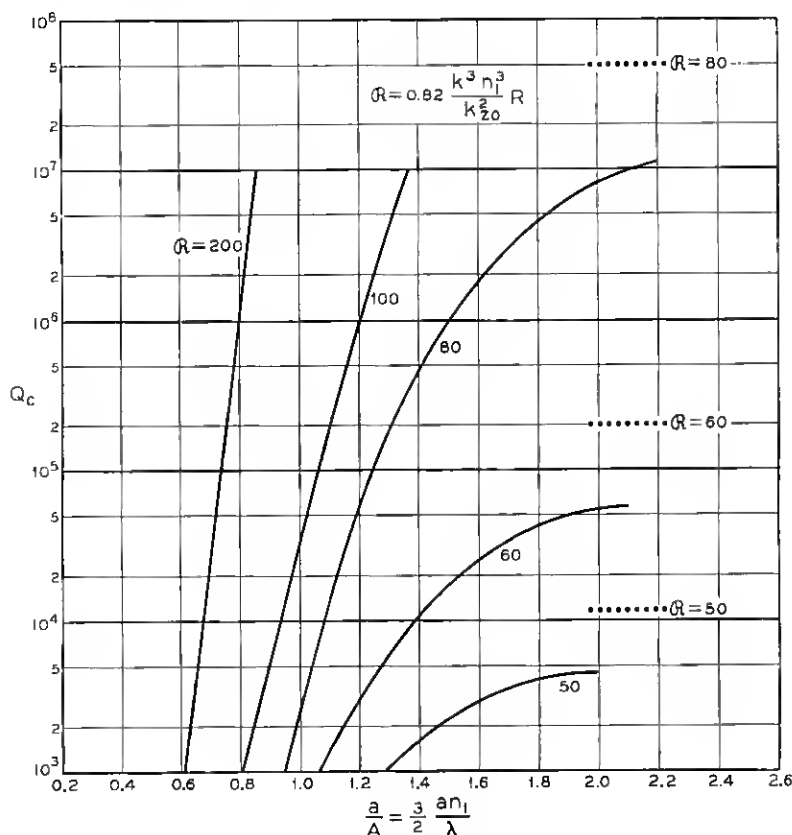
Fig. 8 — Intrinsic Q for E_{11}^y mode if n_1/n_s = 1.5 .
