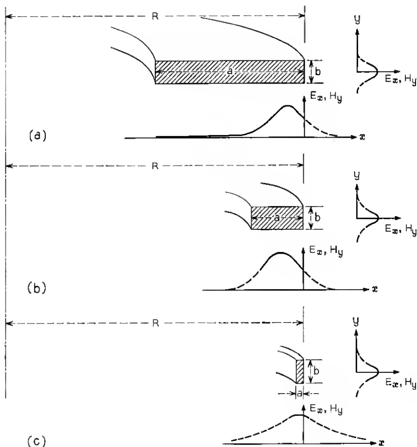
Fig. 6—Field distribution as a function of guide width a with (a) a/A \gg 1 , (b) a/A \cong 1 , and (c) a/A \ll 1 .
